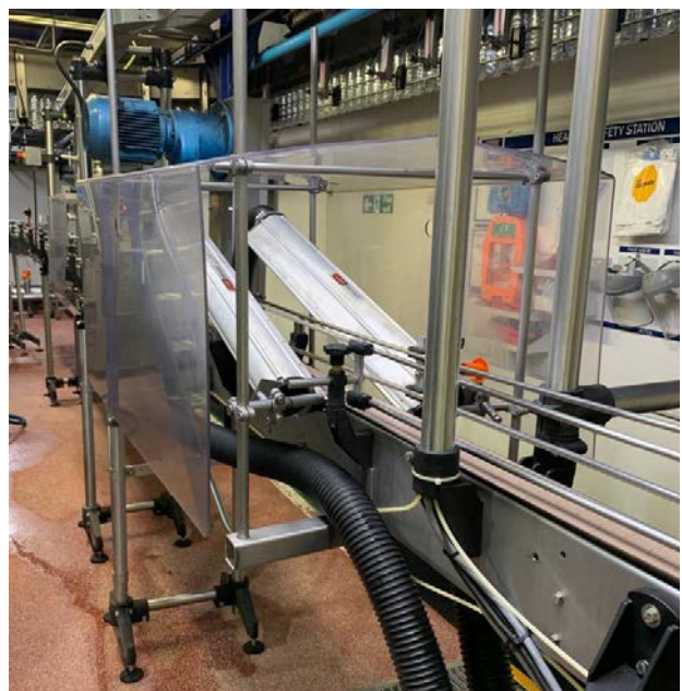
Sonic Air Dryer & Bottle Conveyor
